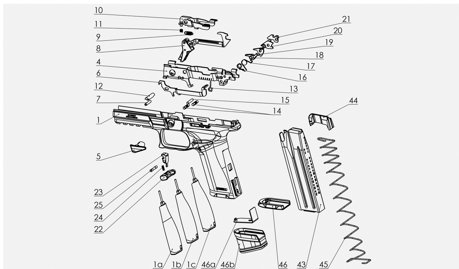
Frame Parts List
